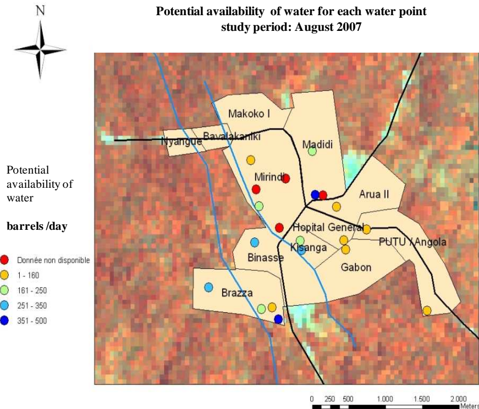
Figure 4. Potential availability of water for each water point, calculated as barrel/ day based on interviews with population
